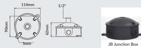
JB Junction Box
