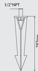
GS Ground Stake Material: PC
