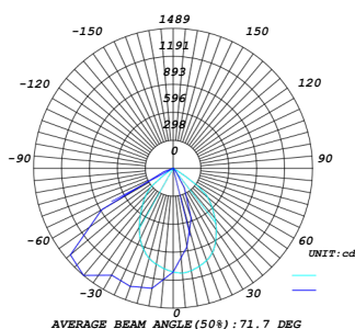
INTENSITY DISTRIBUTION DIAGRAM IN C PLANS
