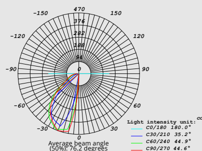
Polar Coordinate Light Distribution Curve
