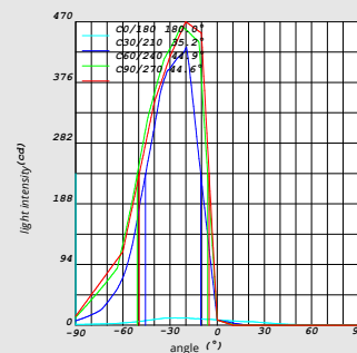
Cartesian coordinate light distribution curve
