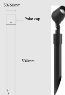
GS Ground Stake 1.1 Material: PVC *Can be customized in different lengths
