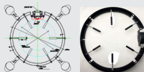
TM Tree Mount 2.0 Material: 304 stainless steel ring + die-casting aluminum waterproof box
