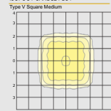
ISOFOOT CANDLE PLOT Type V Square Medium
