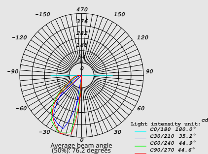
Polar Coordinate Light Distribution Curve
